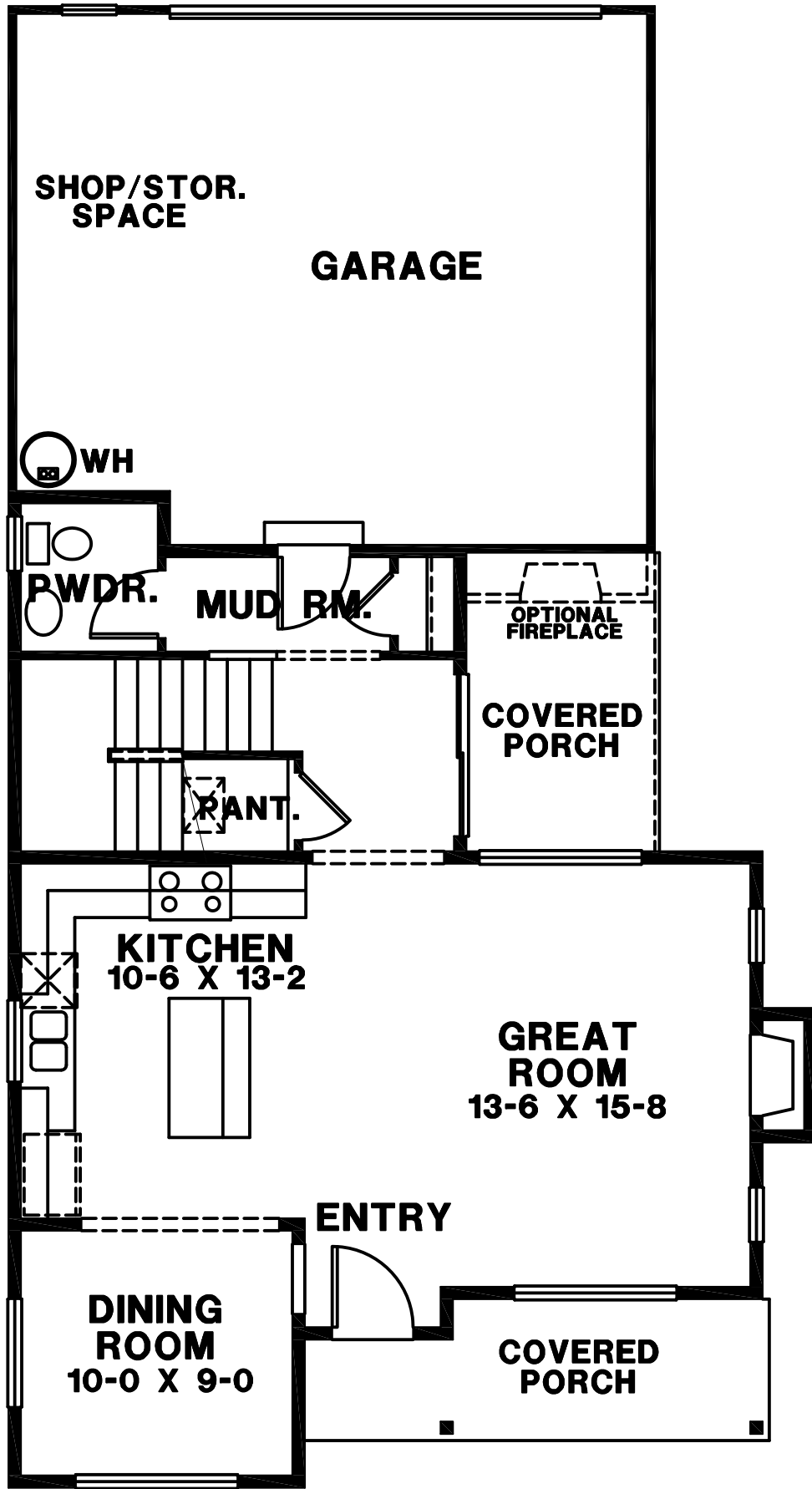
MAIN FLOOR
