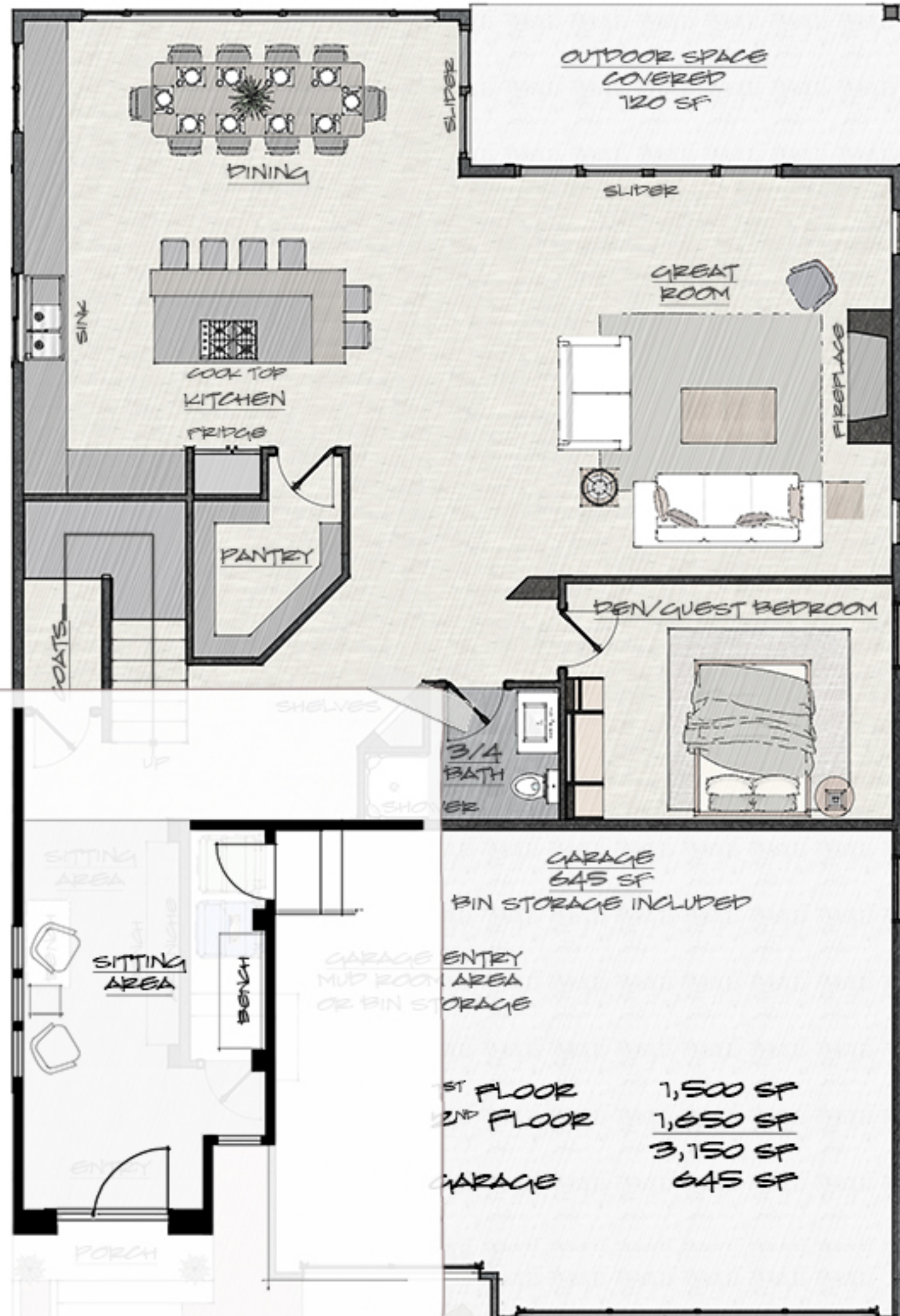
Floor Plan - 1 not to scale
