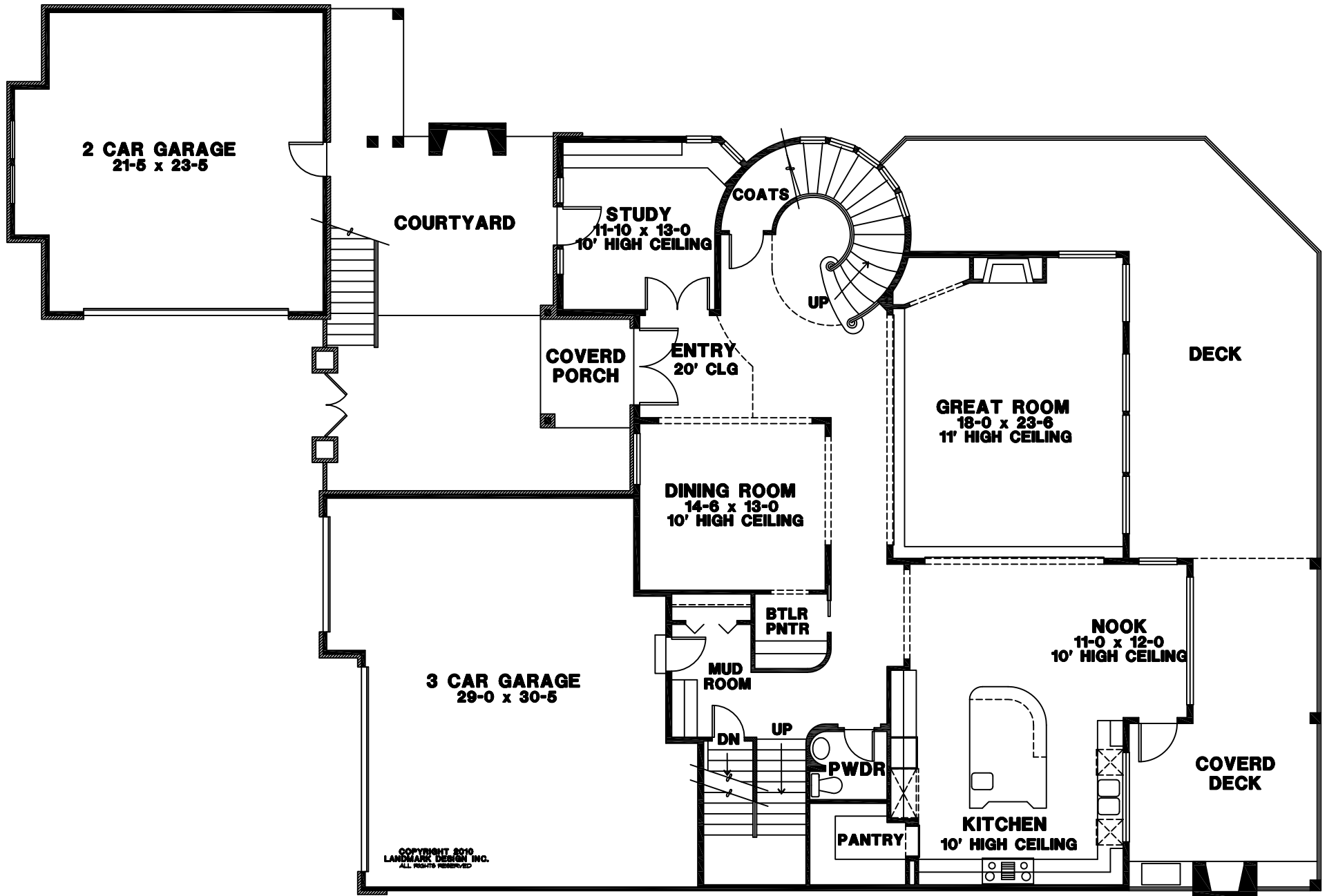
MAIN FLOOR
