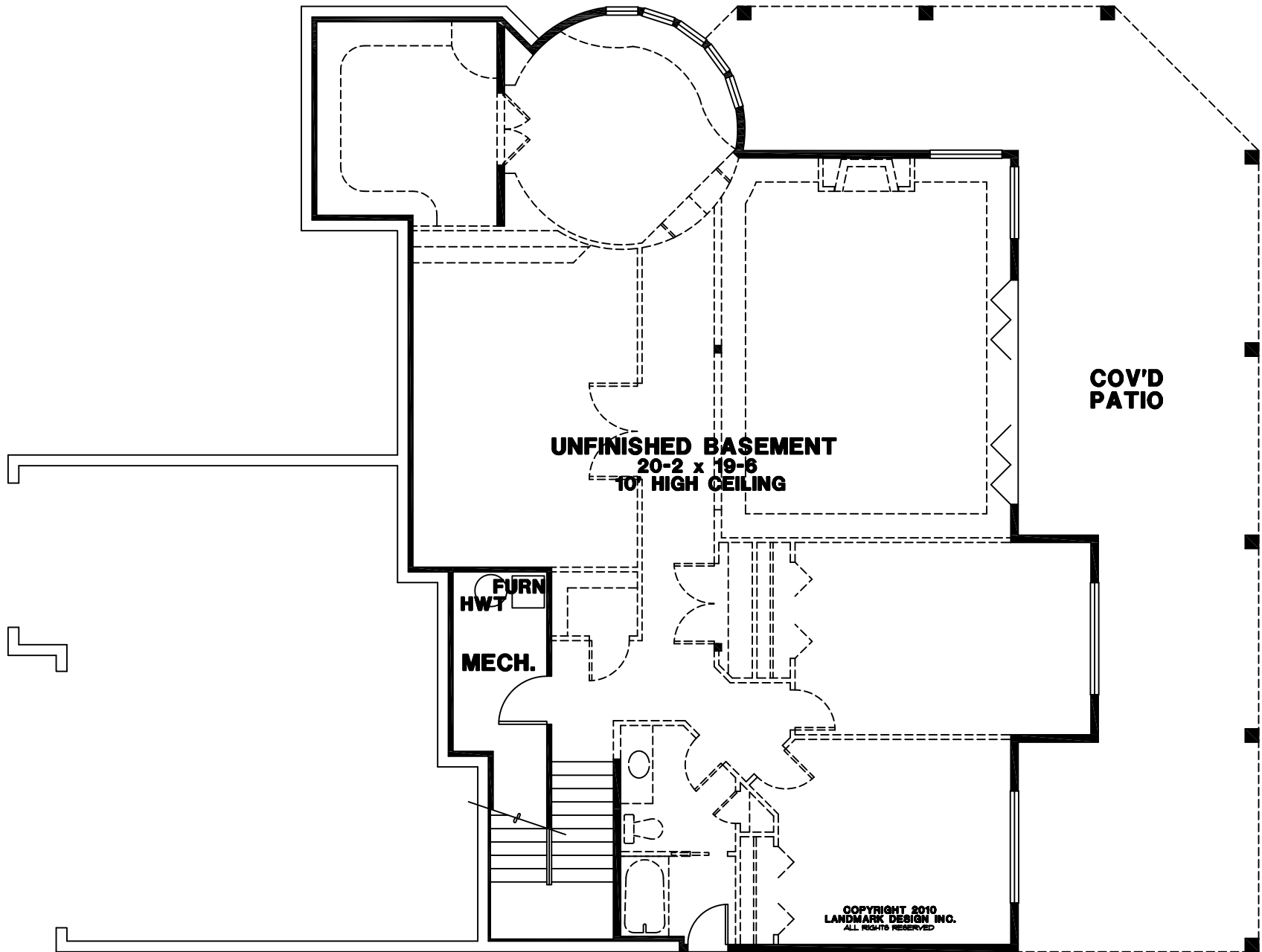
LOWER FLOOR
