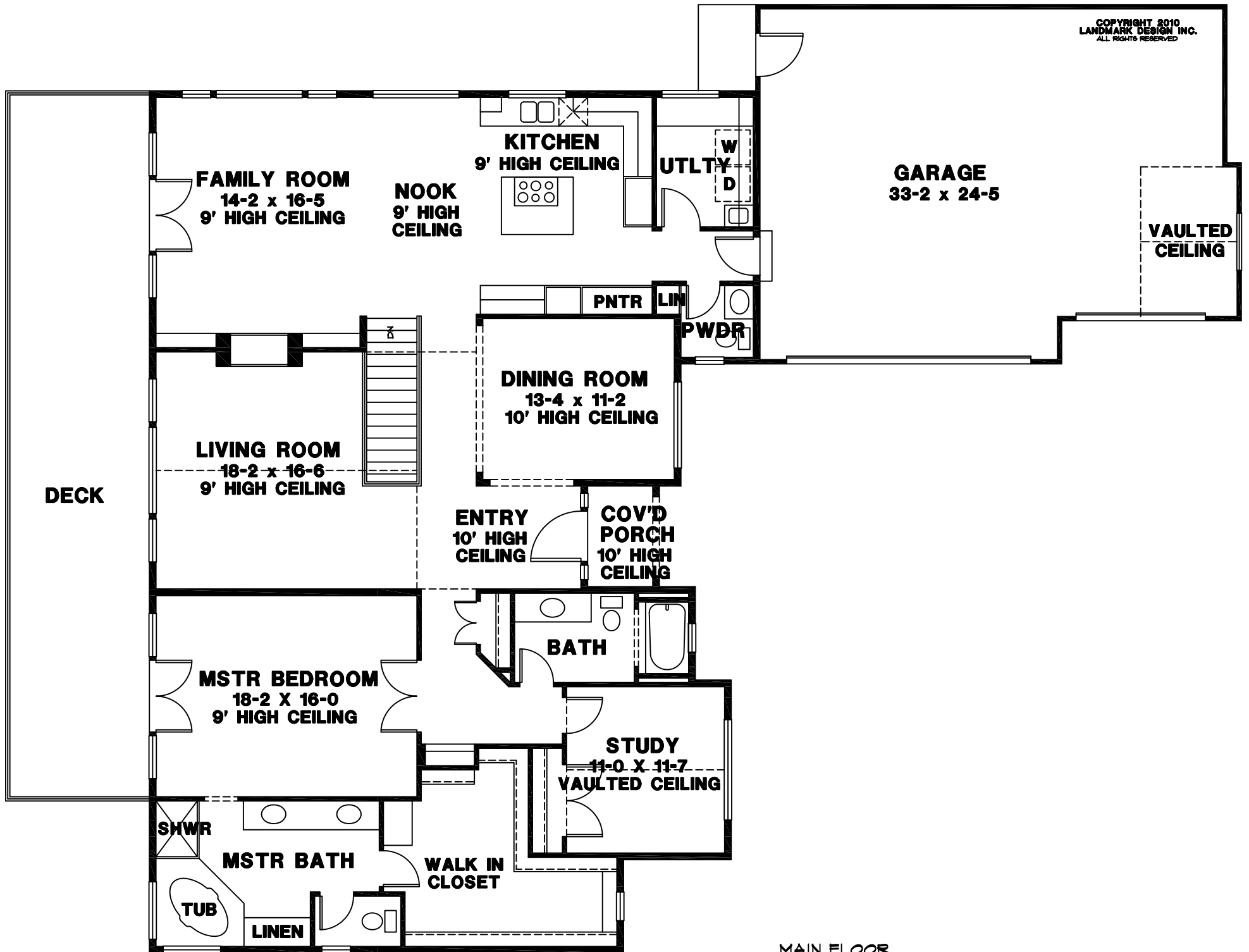
MAIN FLOOR
