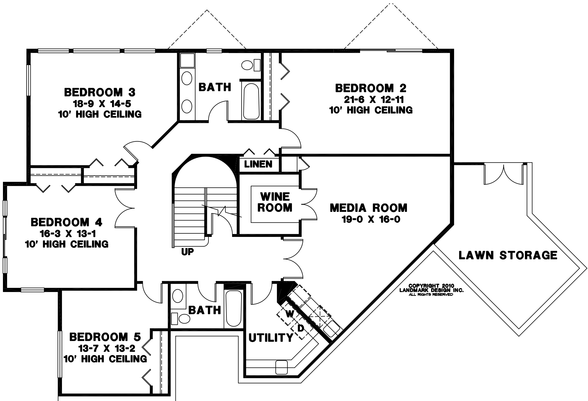
LOWER FLOOR PLAN
