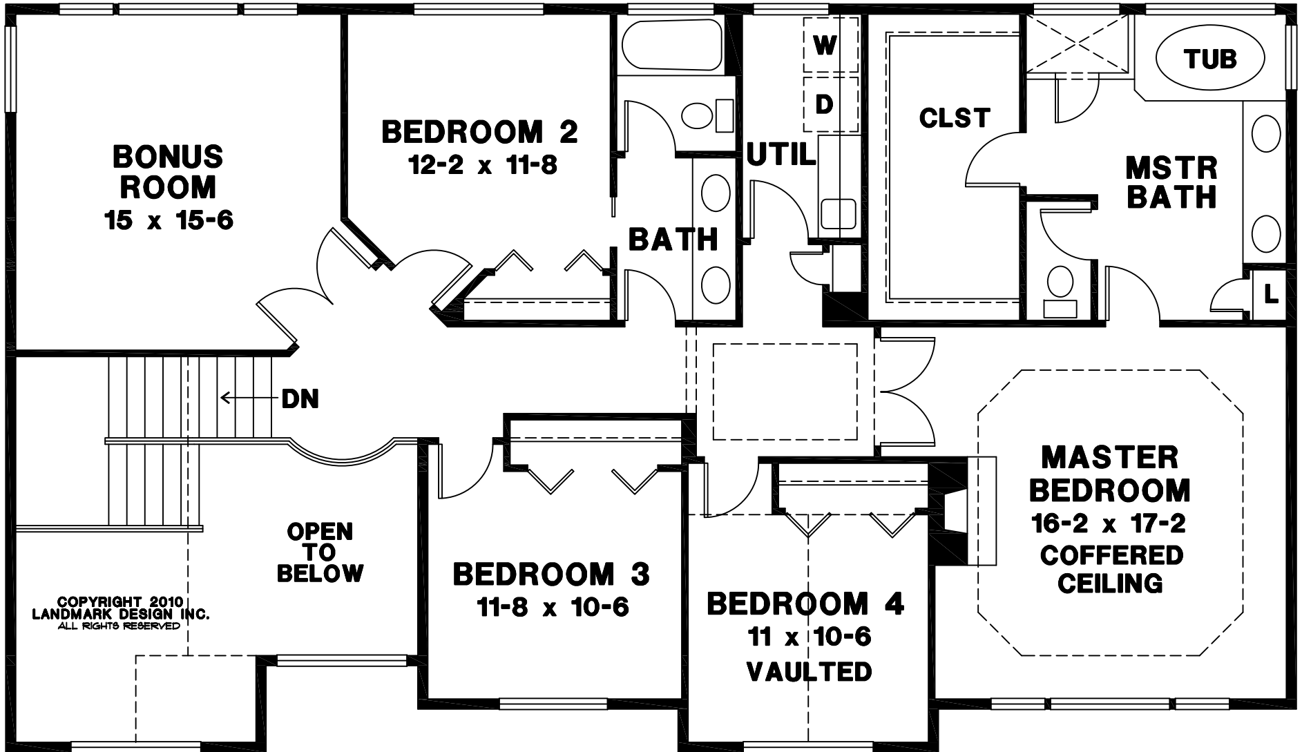
UPPER FLOOR
